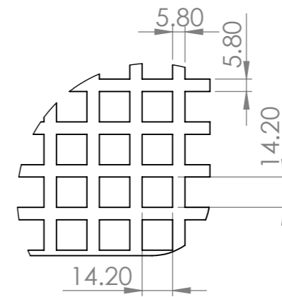
DETAIL A SCALE 2 : 5
